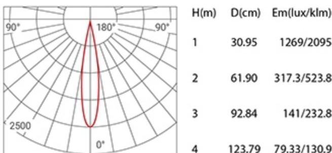
Beam Angle 15° 6W 3000K
