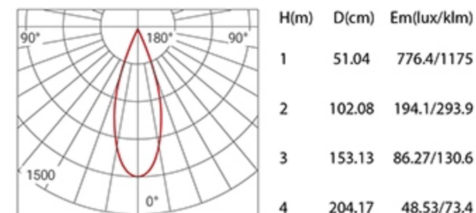
Beam Angle 38° 6W 3000K
