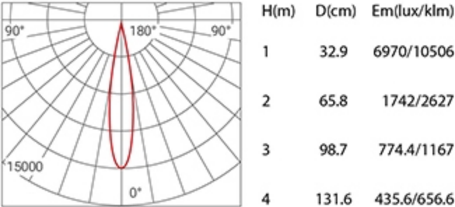
Beam Angle 15° 30W 3000K
