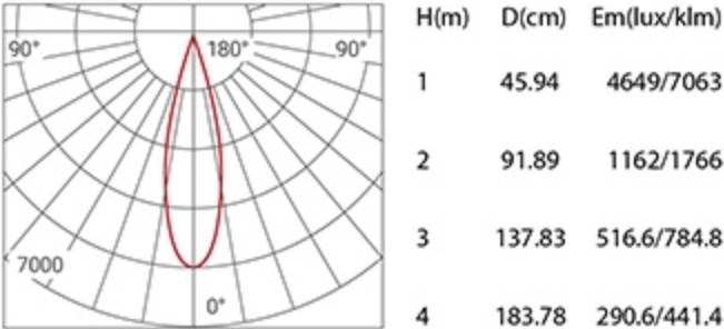
Beam Angle 24° 30W 3000K
