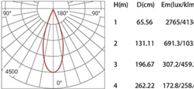
Beam Angle 38° 30W 3000K
